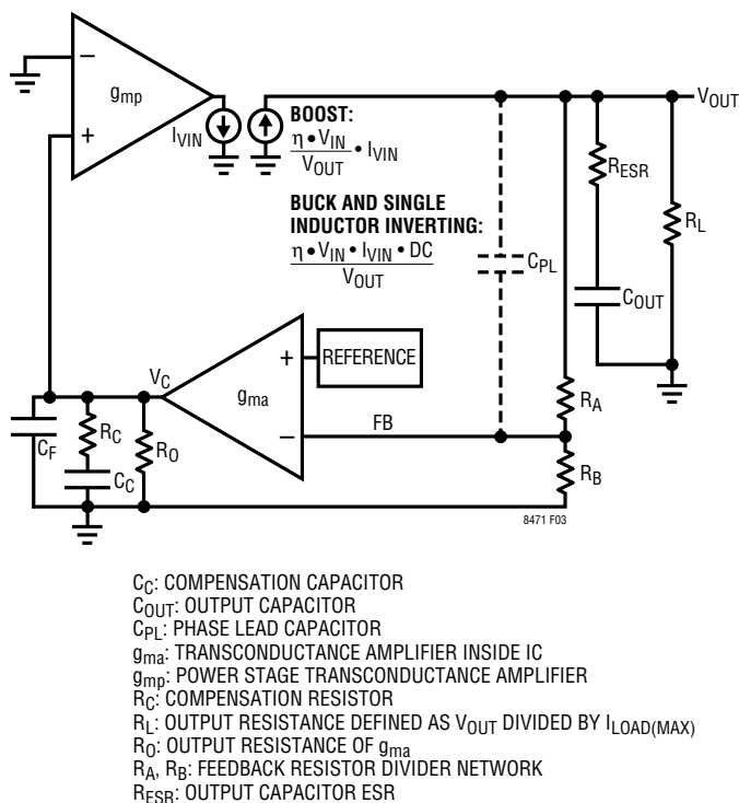
Figure 3. Boost/Buck/Inverting Converter Equivalent Model
